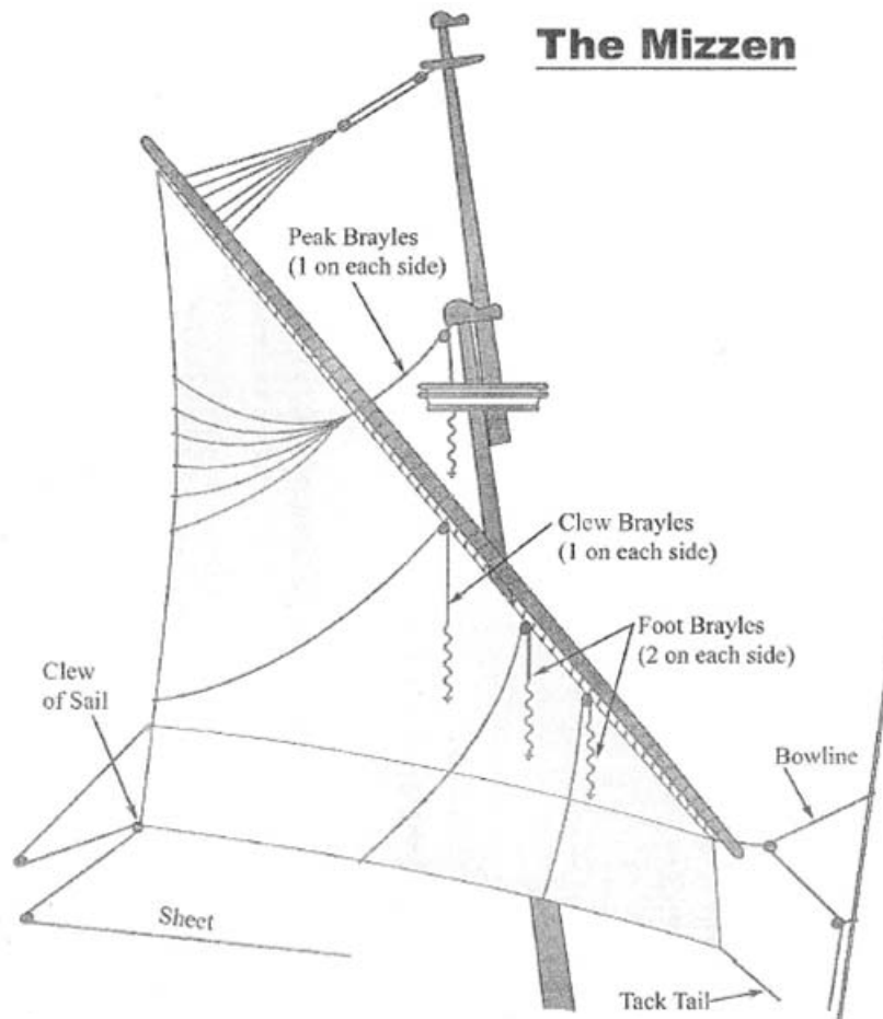
Figure 2.15 Labeled Running Rigging of the Mizzen
