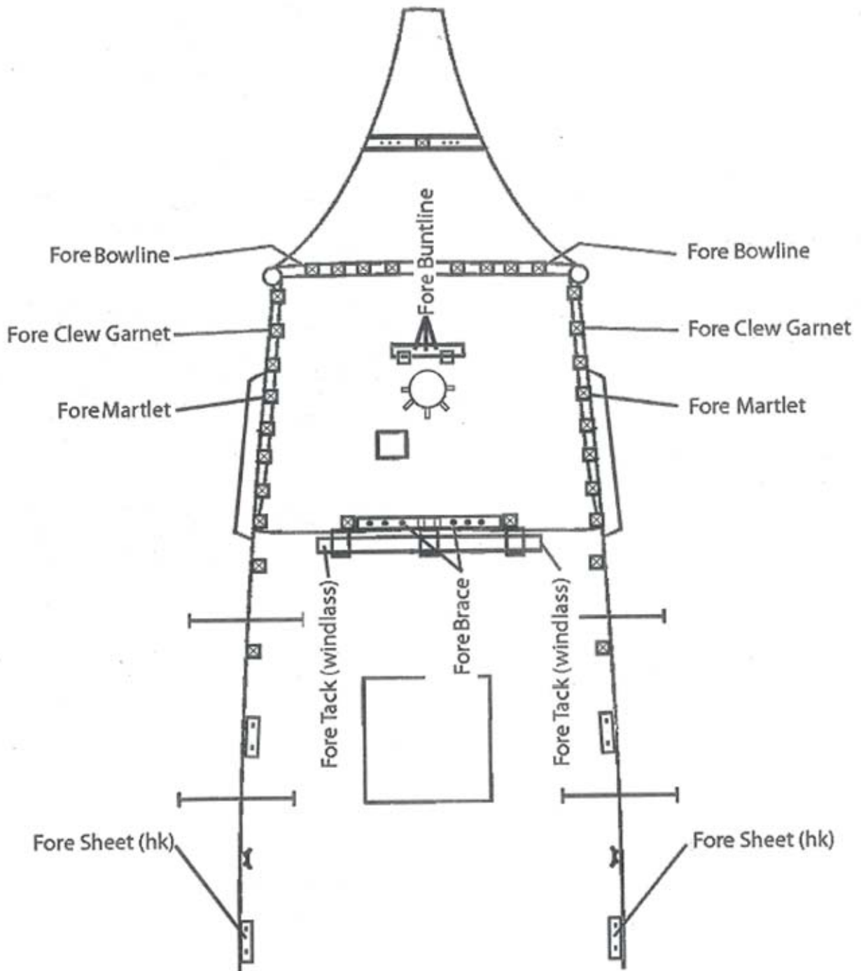
Fore Course Belay Diagram
