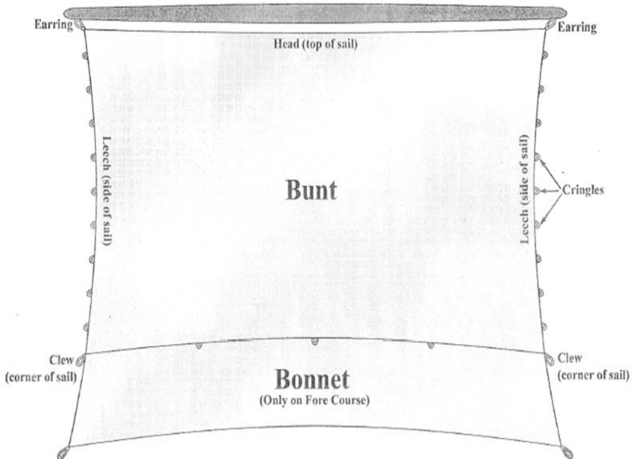
Figure 2.10 Labeled Parts of a Course
