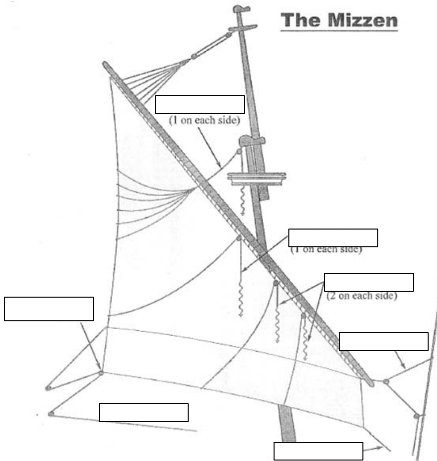
Figure 2.15 Labeled Running Rigging of the Mizzen
