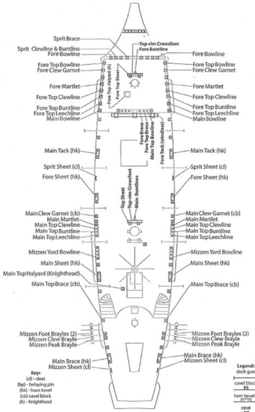
Ordinary Seaman Belaying Diagram
